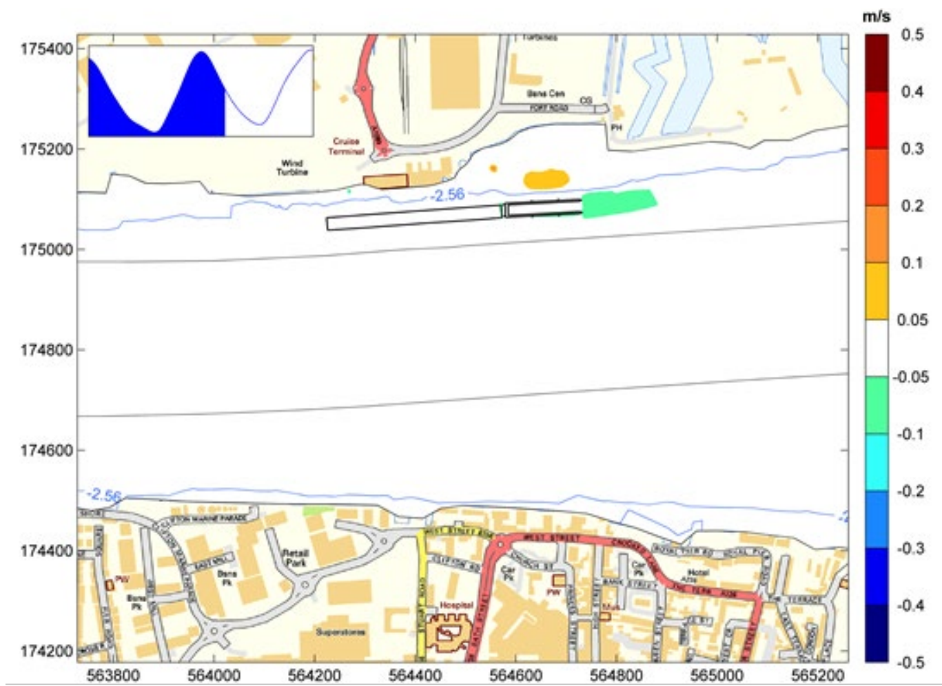
Figure 17.31: Essex Project Site difference in current magnitude at time of peak ebb tide against the baseline model.
